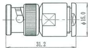
BNC-P-5
