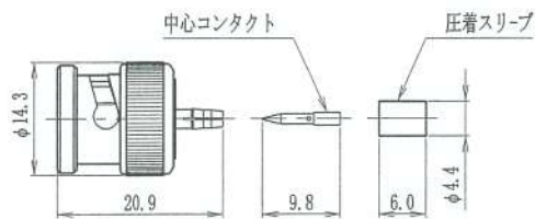
BNC-GP2-1.5C
