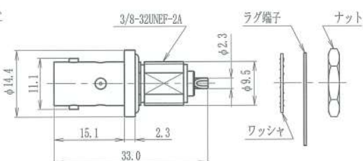
BNC-BR
